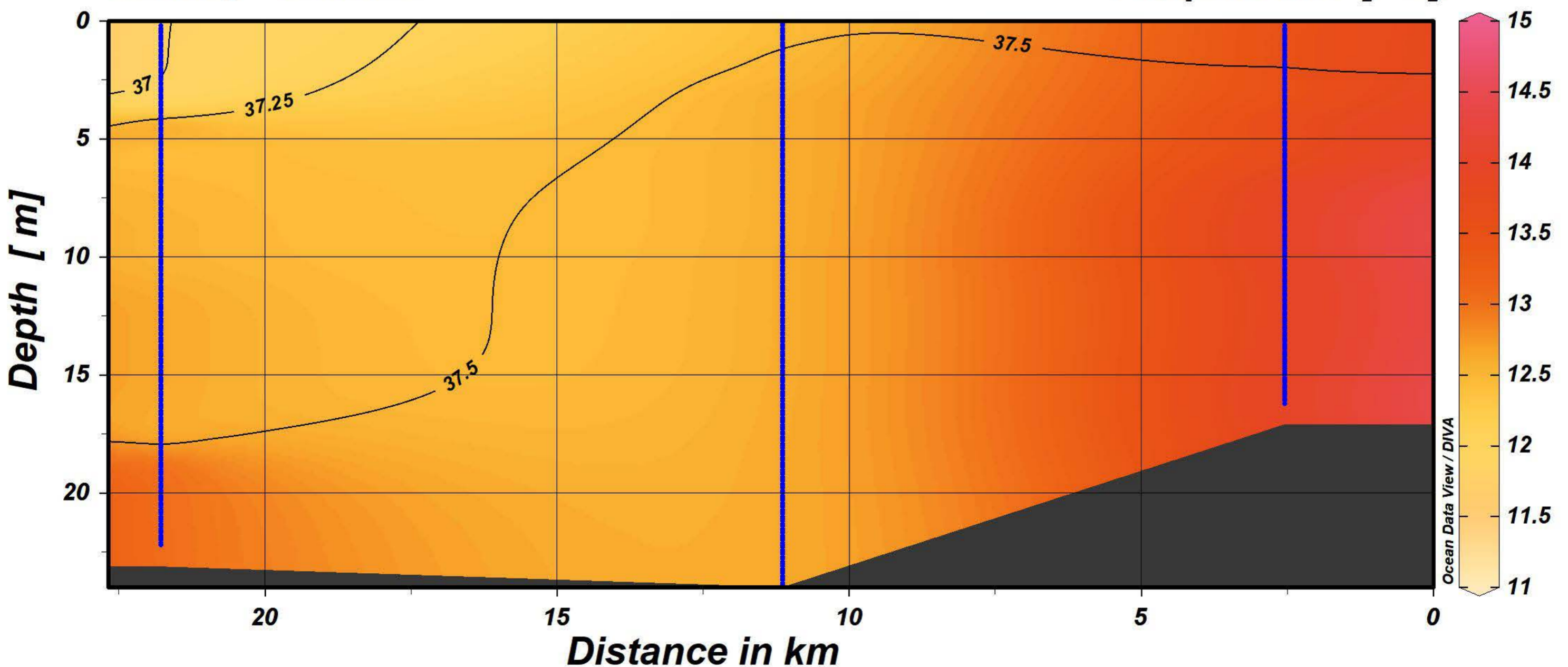
Salinity - isolines
