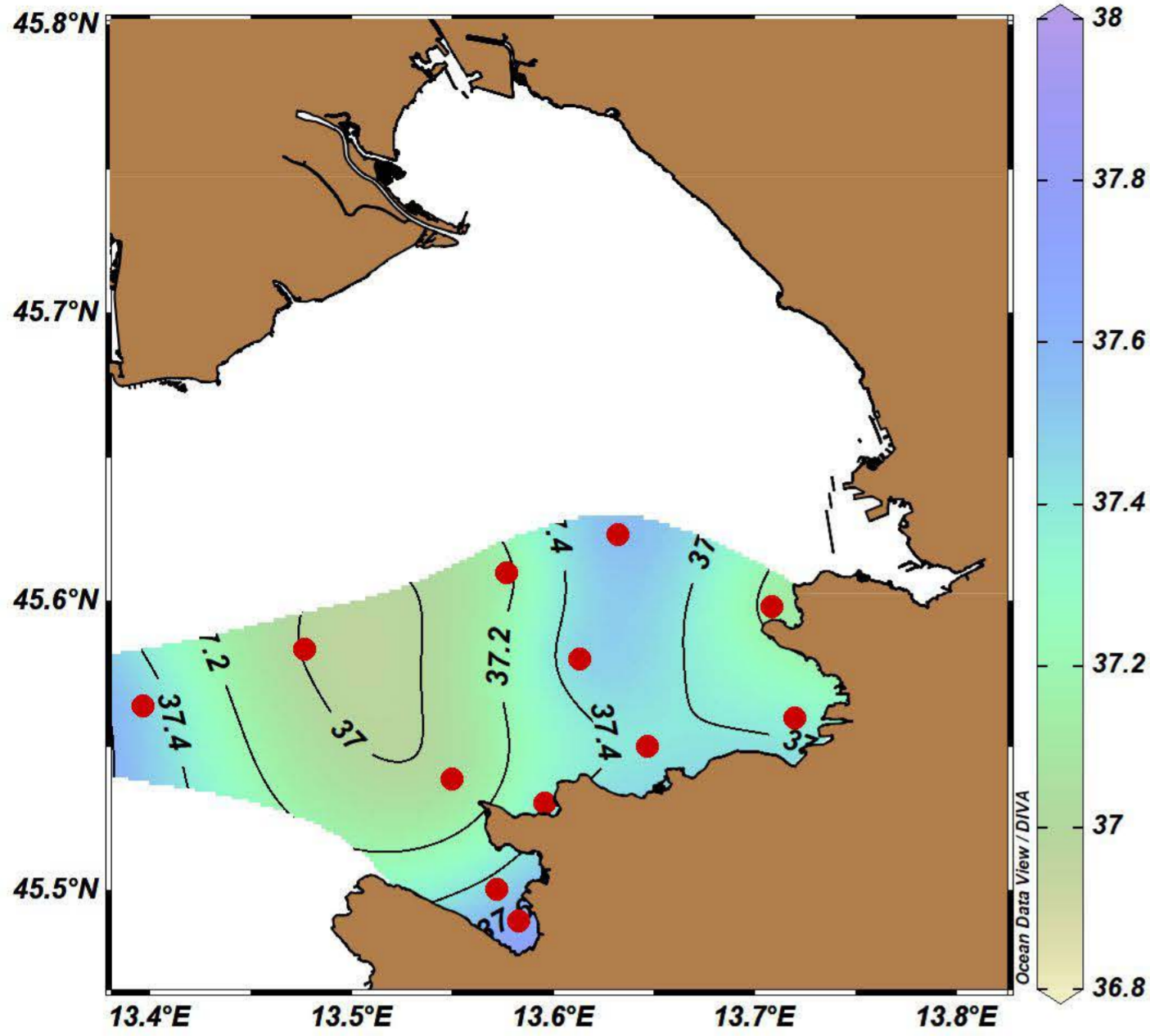
Surface Salinity
