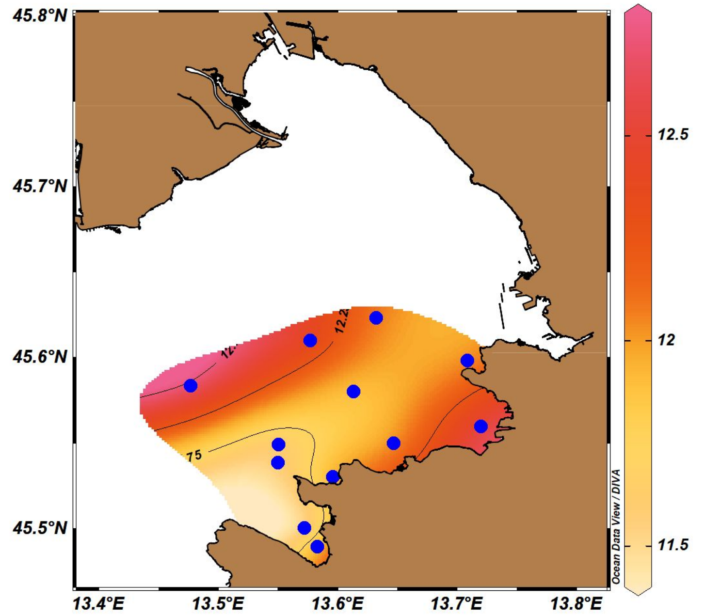
Surface Temperature [ °C]
