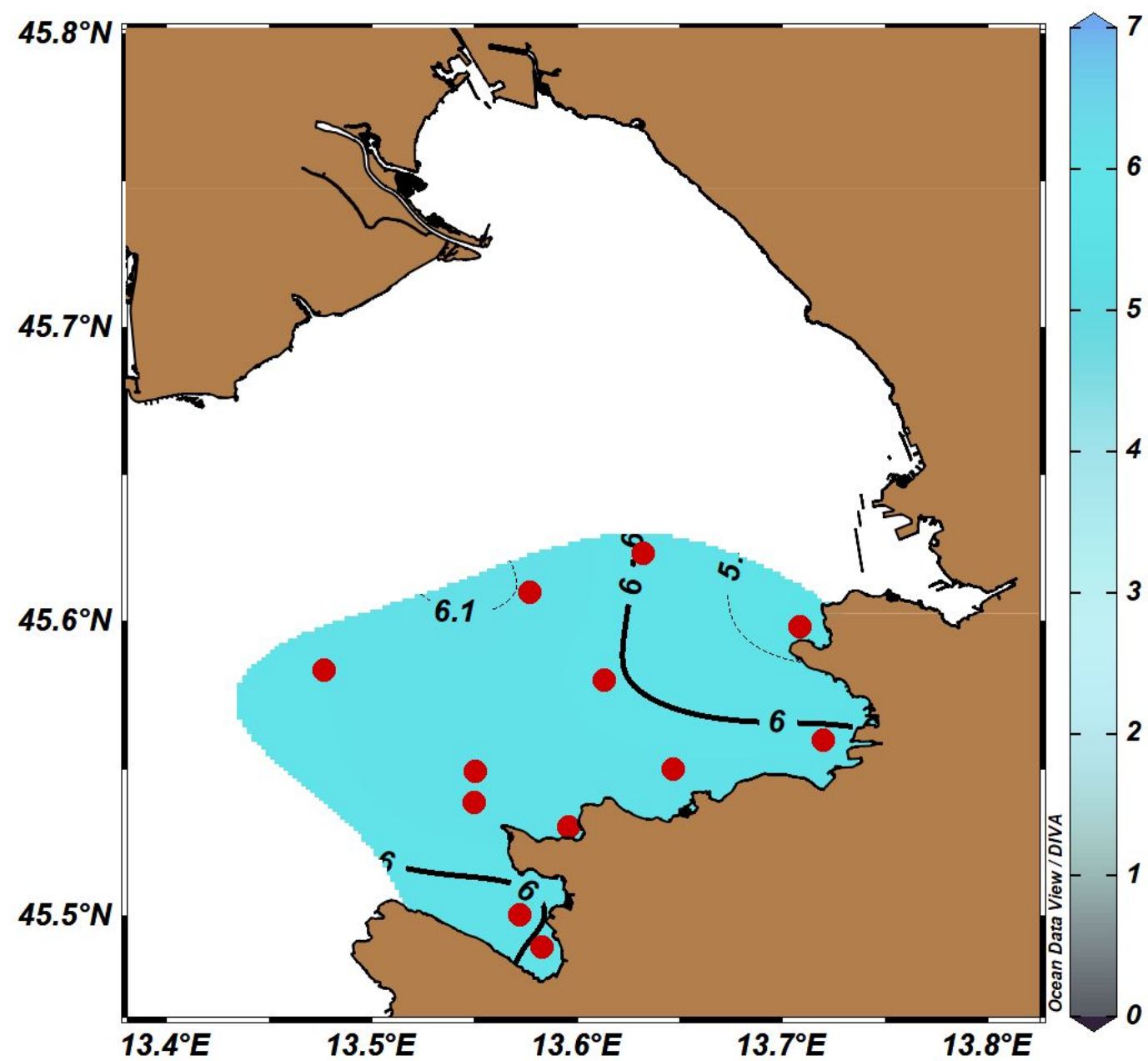
Dissolved Oxygen at the bottom [ml/l]
