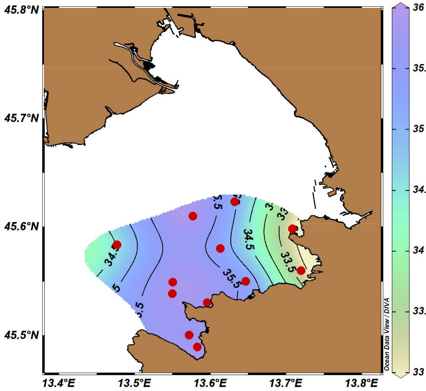
Surface Salinity
