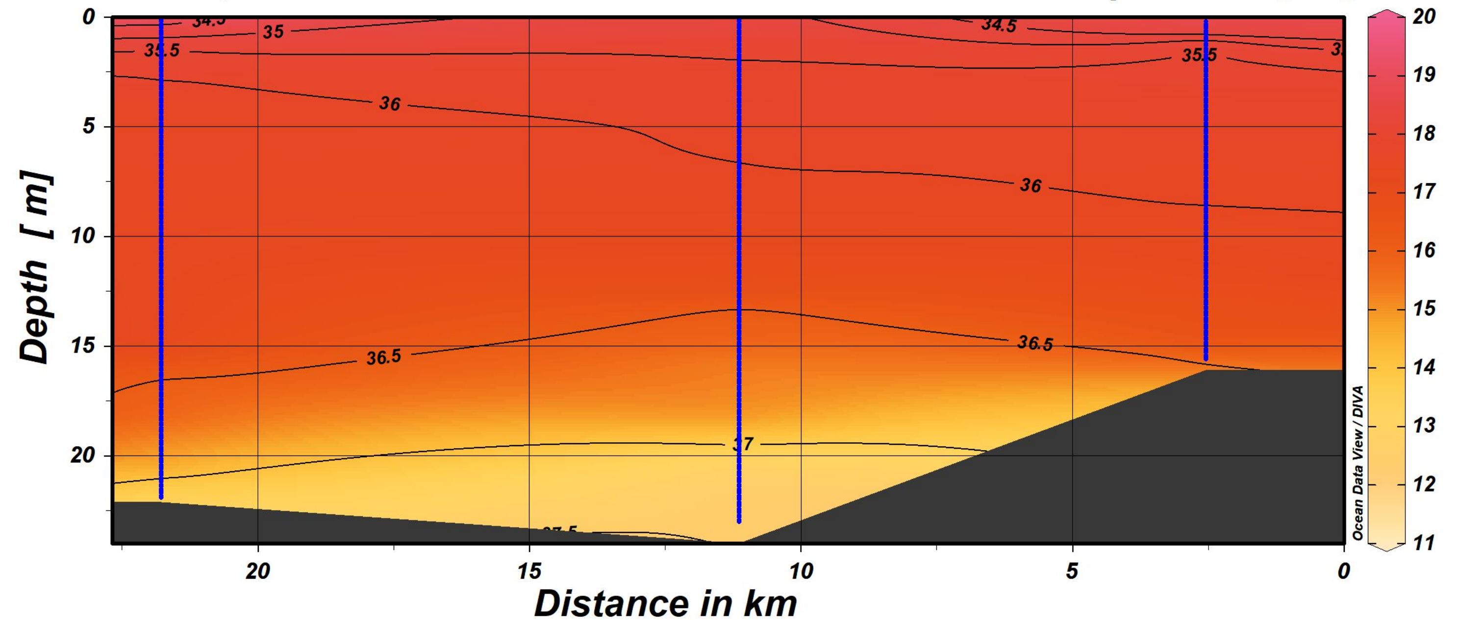
Salinity - isolines
