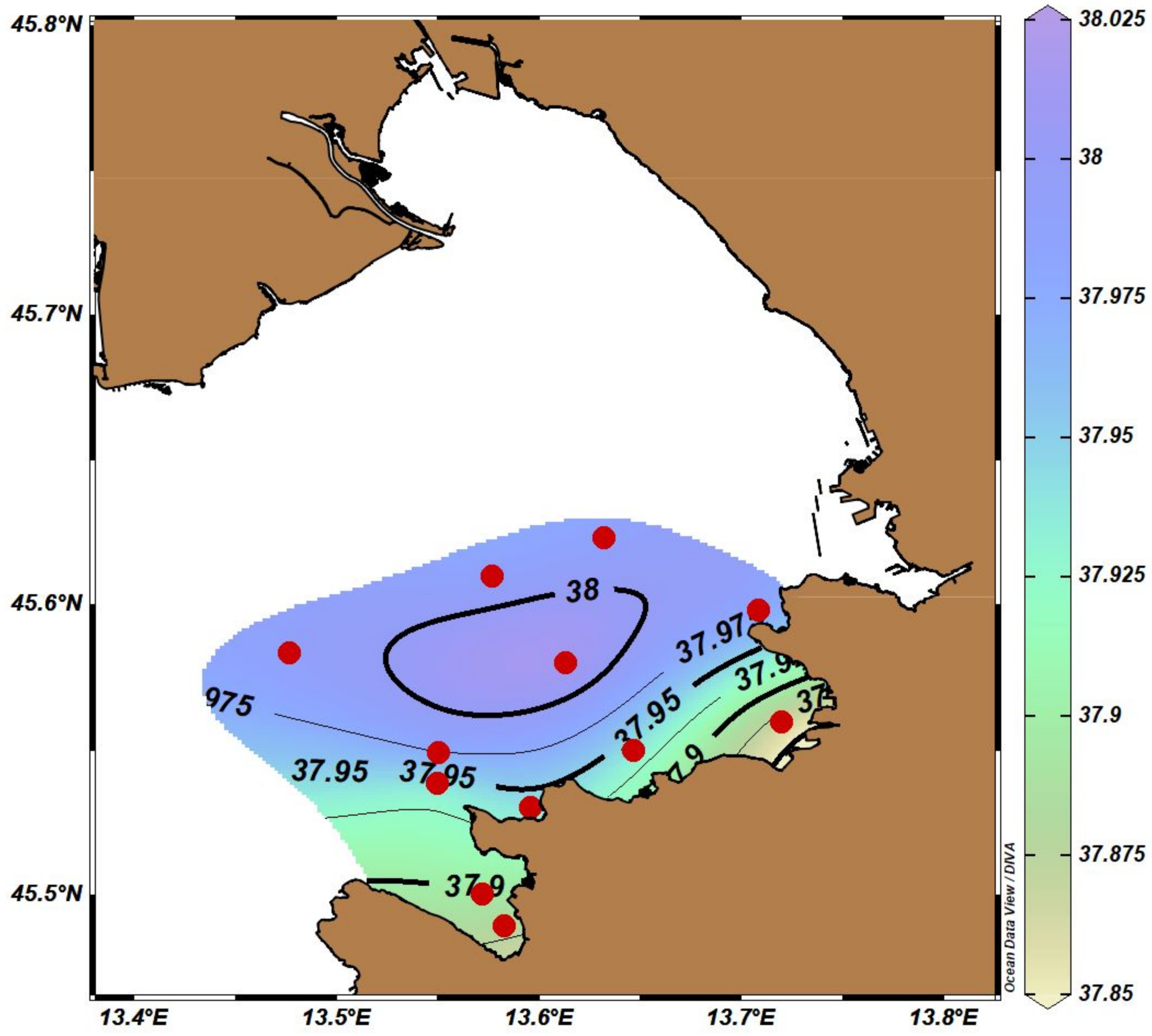
Surface Salinity
