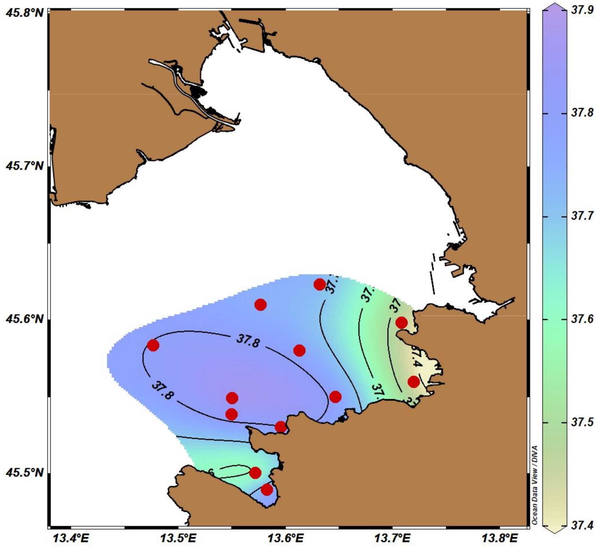
Surface Salinity
