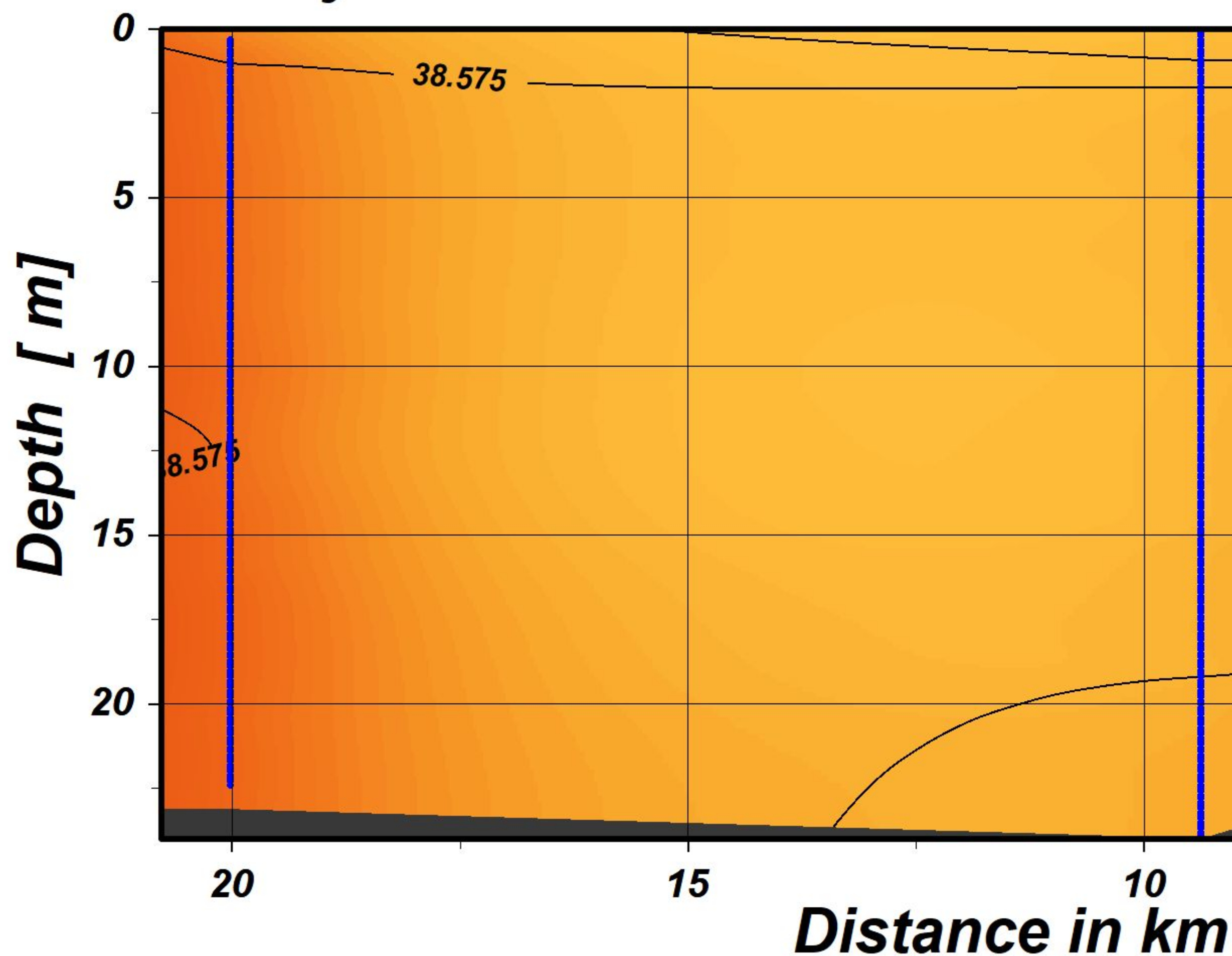
Salinity - isolines
