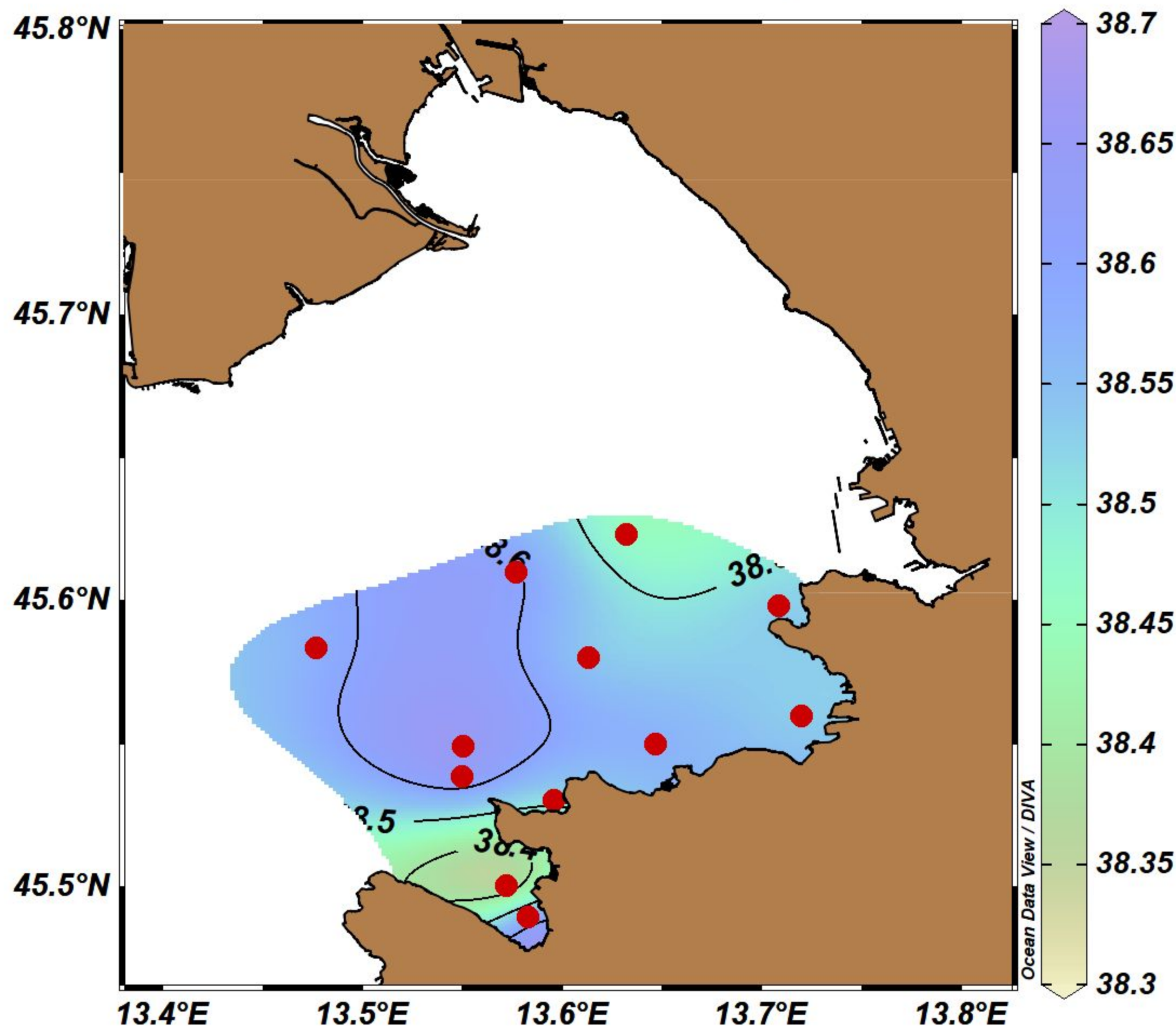
Surface Salinity
