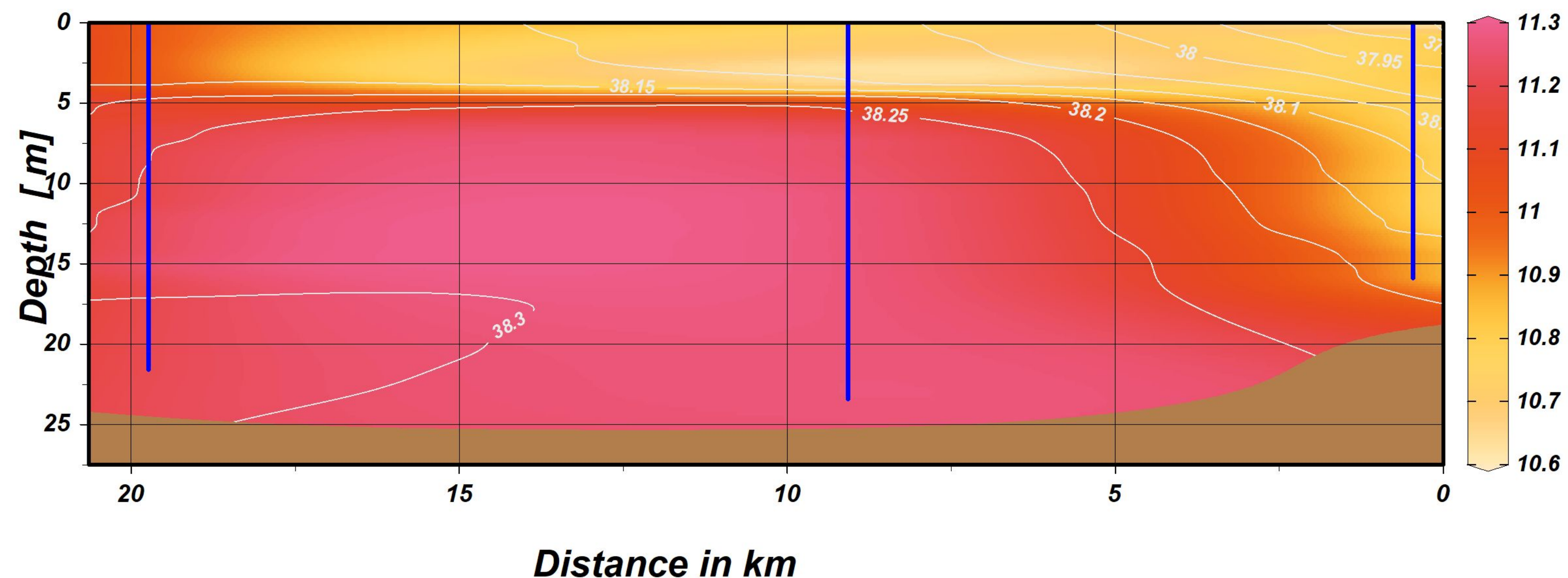
Salinity - isolines
