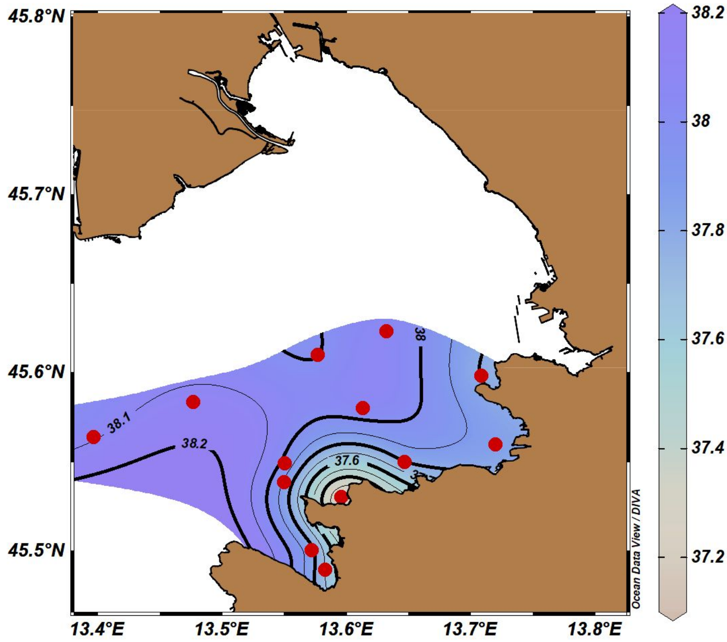
Surface Salinity
